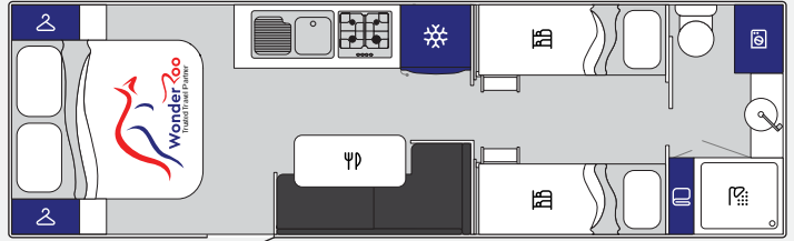
24'6" QUAD BUNK
