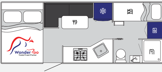
19'6" DOUBLE/TRIPLE BUNK
