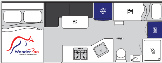
20'6" DOUBLE OR TRIPLE BUNK
