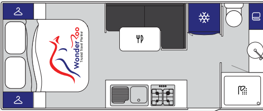
19'6" COUPLES
